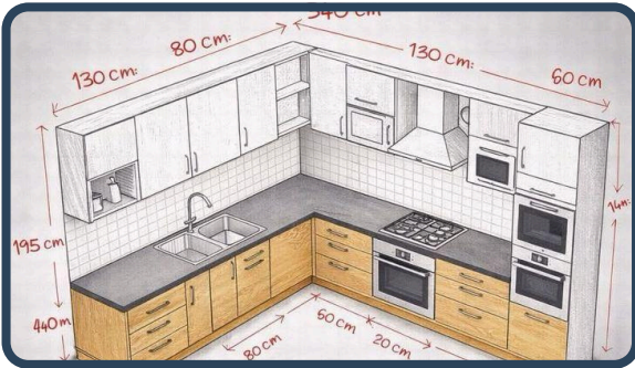
2D Design
